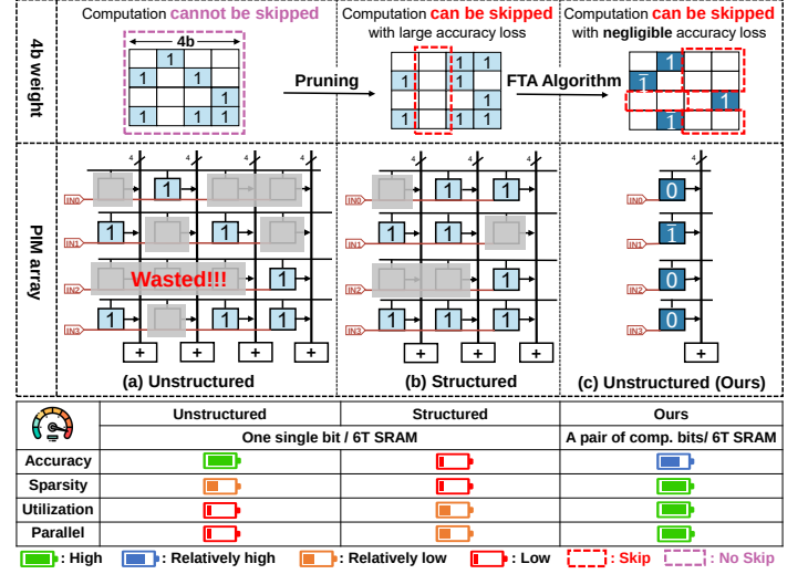
Figure 1: Exploitation of bit-level sparsity in SRAM-PIMs.
